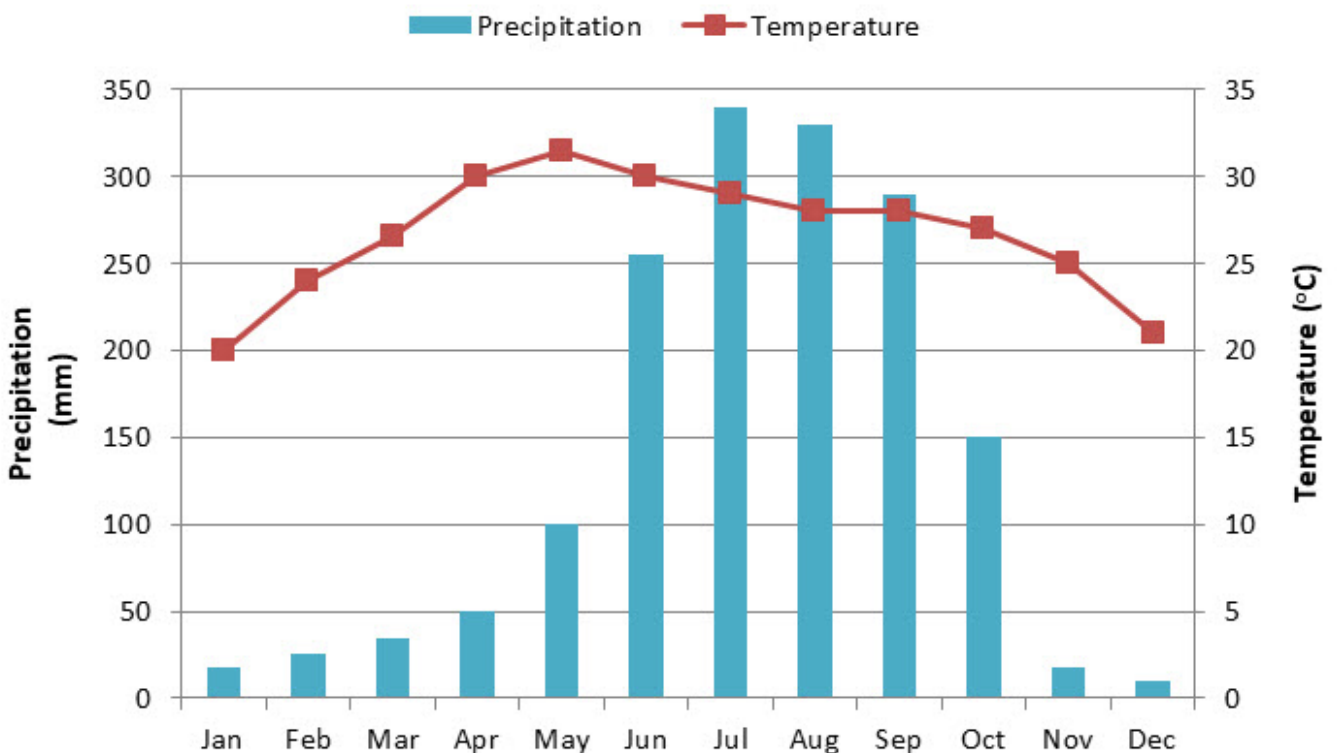
Monthly Temperature and Precipitation
